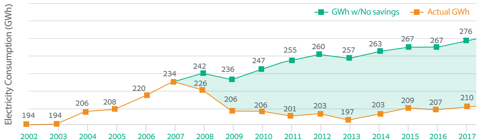
Overall Electricity Consumption and Savings 2002-2017, in GWh
